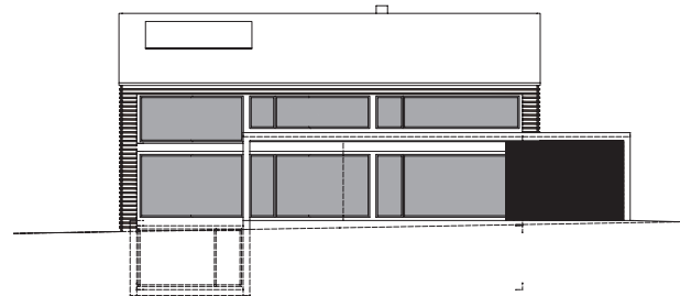
Elevation South-East
