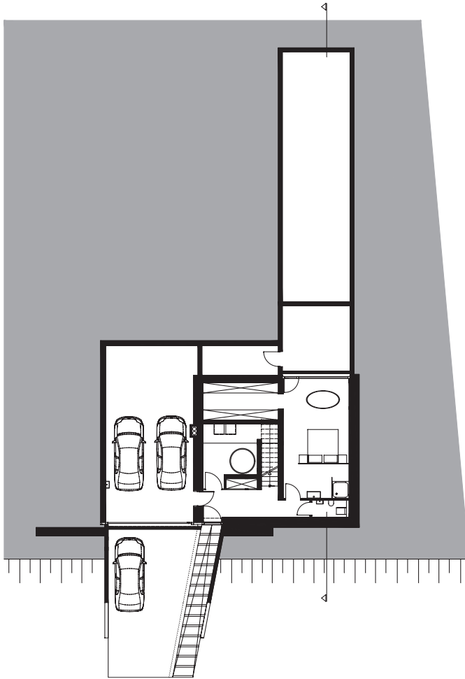
Basement Floor
