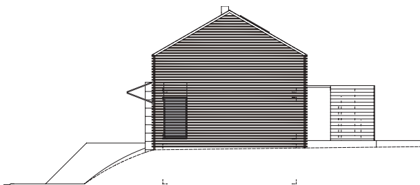
Elevation South-West
